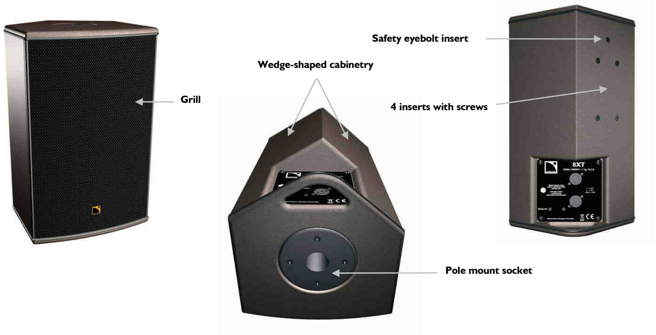
Figure 3: The 8XT enclosure
